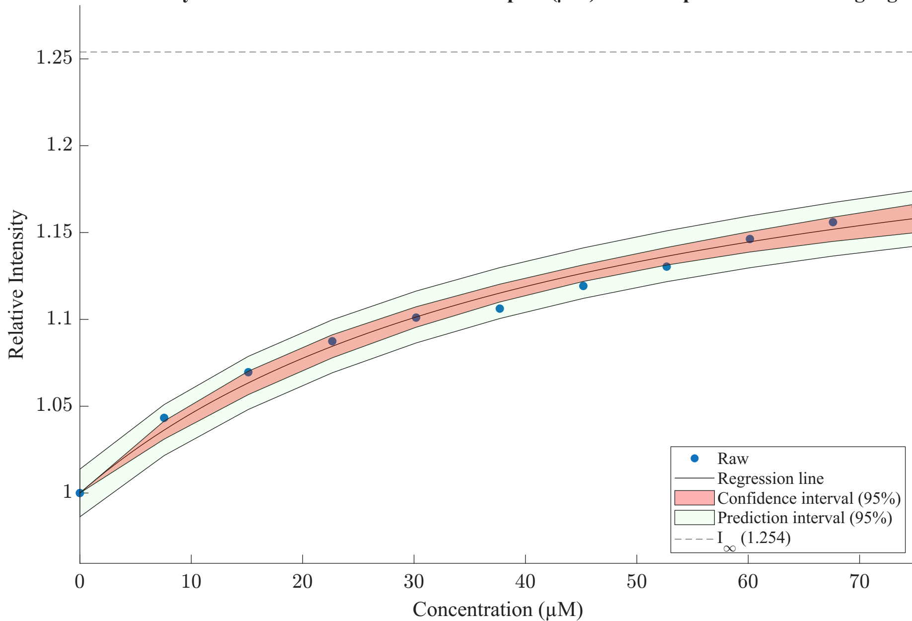
Relative intensity as a function of concentration of lipids ( \mu\text{M} ) for l8r rep3 - Statistics fitting algorithm
